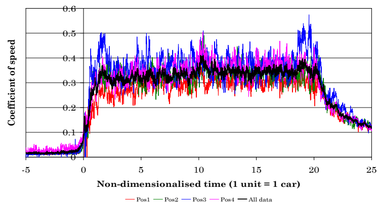
Figure 34 Ensemble average normalised velocities beneath a 20 car Class 373 Eurostar at different points across the track (9) (The x axis shows distance along the train normalised with the length of an average car, and the y axis shows horizontal velocity normalised with train speed.)
