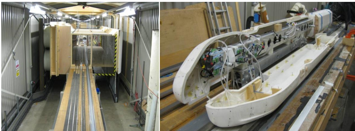
Figure 11 TRAIN Rig cross wind generator and instrumented train showing train mounted pressure transducers (28)
