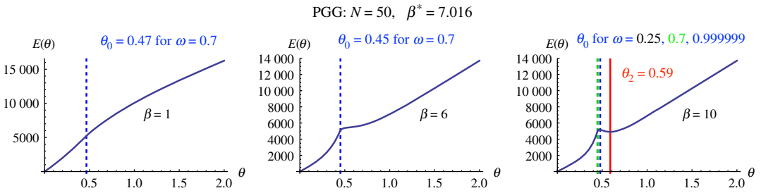
Figure 4. We use algorithm 3.3 to find optimal \theta that minimizes E(\theta) while ensuring a minimum level of cooperation \omega , for PGG ( r = 3, n = 5, c = 1 ) with N = 50 . Similar observations to those for DG are obtained. (Online version in colour.)
