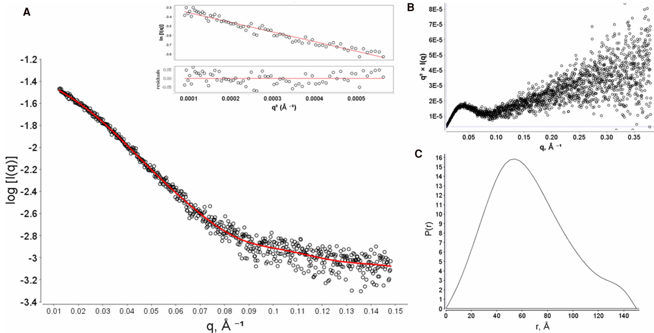
Figure 5. Small angle X-ray scattering analysis of Sav186-SMALPs.
