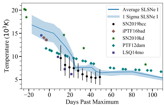
Figure 7. Temperature comparison of SN 2019hcc with a small sample of SLSNe I. The closest SLSN I in temperature to SN 2019hcc at the epoch of +7 days is LSQ14mo. The SLSN temperatures are taken from the literature (see text). The average temperature for SLSNe I is taken from Inserra et al. (2017) and reference therein.
