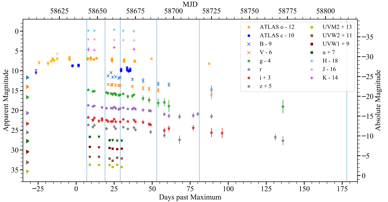
Figure 5. Photometry for SN 2019hcc - the light curves from various sources: BVgri bands were taken by LCO, and griz bands were also taken by LT. Alongside this, there is ATLAS data including the pre-peak limits, Swift UV data, and GROND NIR data. The vertical lines mark the epochs when the spectra were taken. The markers on the left y-axis signify the galaxy magnitude in the respective bands.
