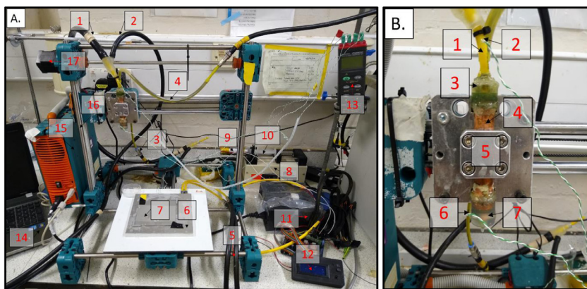
Fig. 1. Schematic of the retrofitted Fabbster printer (A) including (1) Jacketed pipe from the syringe to the nozzle, (2) Jacketed pipe from the nozzle to the water bath, (3) Jacketed pipe from a water bath to the bottom of the nozzle, (4) Pipe from the top of the nozzle to the water bath, (5) Jacketed pipes to and from a water bath to the temperature controlled bed, (6) Temperature controlled printing bed (7) Removable section of the printing bed (8) Syringe driver, (9) Heating jacket, (10) 60 mL syringe, (11) Power supply unit, (12) Controller for heating jacket, (13) Data logger, (14) Laptop to control printer, (15) Controller unit for the printer, (16) Support rods for the printer, (17) Support rods and motor for the printer. (B) Schematic of the printer nozzle including (1) Feed pipe into the nozzle, (2) Thermocouple to monitor temperature of feed material as it enters the nozzle, (3) 3D printed part to connect feed pipe to the copper pipe, (4) Copper outer pipe containing brass inner pipe, (5) Bracket to hold copper pipe
