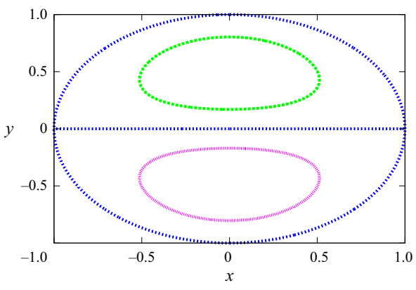
Figure 5. Streamlines for the Lamb–Chaplygin dipole (4.13).
