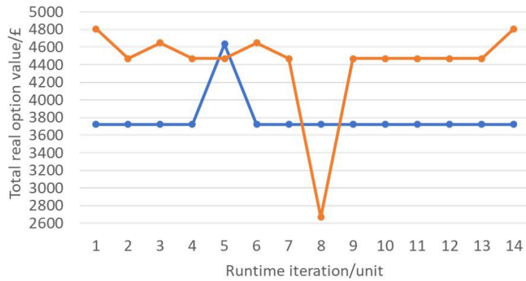
Fig. 4. Corresponding output of our process over same time period as in Figure 3; 1 runtime iteration = 5 milliseconds; the blue line refers to the real option values of adapting granularity while the orange line refers to the real option values of keeping the granularity level unchanged
