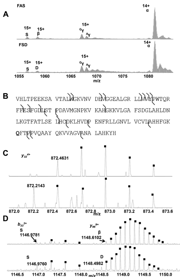
Figure 3. (A) SIM mass spectra of normal neonate Hb heterozygous and homozygous FAS (top) and FSD (bottom). (B) CID sequence coverage of heterozygous FSD (variant HbD) ions only). (C) Expanded m/z region showing the y_{32}^{4+} fragments observed following CID of the \beta -chain ions ( m/z_{\text{calc}} 1307.9266; top) in the FAS sample and HbD variant ions ( m/z_{\text{calc}} 872.2140; bottom) in the FSD sample. (D) Expanded m/z region showing both the b_{33}^{3+} fragments observed following CID of the HbS variant ions ( m/z_{\text{calc}} 1146.9751) and the y_{96}^{9+} fragment ions of the \beta -chain ions ( m/z_{\text{calc}} 1148.6083) and HbD variant ions ( m/z_{\text{calc}} 1148.4982).
