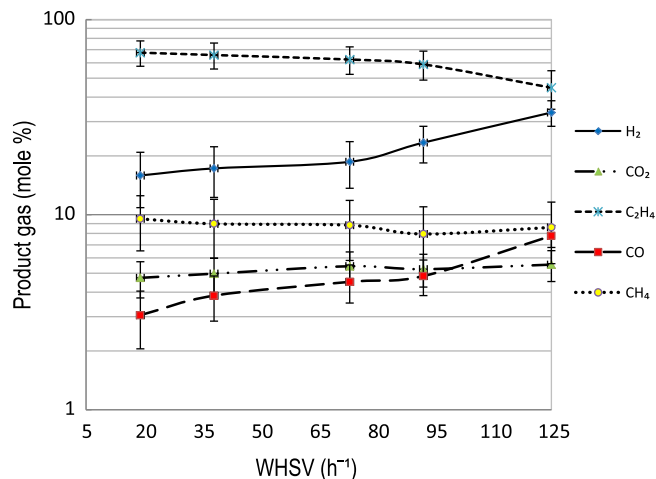
Fig. 6. Effect of WHSV on CSCWG of 20 wt% glycerol. T = 500 °C and P = 250 barg.
