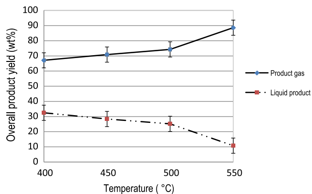
Fig. 9. Effect of temperature on gas-liquid product yields for 10 wt% glycerol. P = 235 barg, WHSV = 125 h -1 . Note gas and liquid yields do not equal 100% as char formed part of the overall product.
