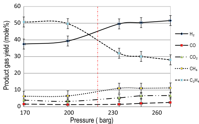
Fig. 7. Effect of pressure on gas product yield for 10 wt% glycerol. T = 500 °C, WHSV = 125 h -1 . Vertical dotted red line indicates supercritical conditions at 221 barg. (For interpretation of the references to colour in this figure legend, the reader is referred to the web version of this article.)
