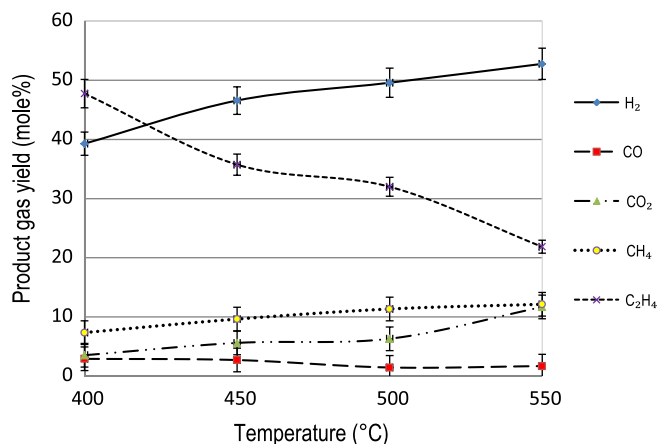
Fig. 8. Effect of temperature on gas products yield for 10 wt% glycerol. P = 235 barg, WHSV = 125 h -1 .
