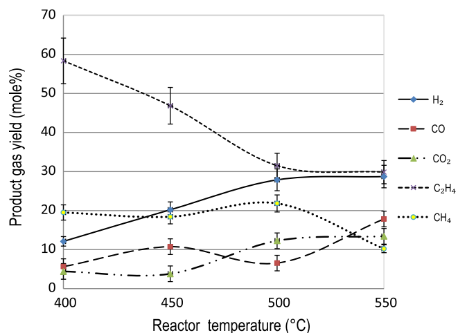
Fig. 5. Gaseous products identified from the non-catalytic SCWG of 15 wt% glycerol. P = 250 barg at F = 65 ml/min, \tau = 28 s, LHSV = 128 h -1 .
