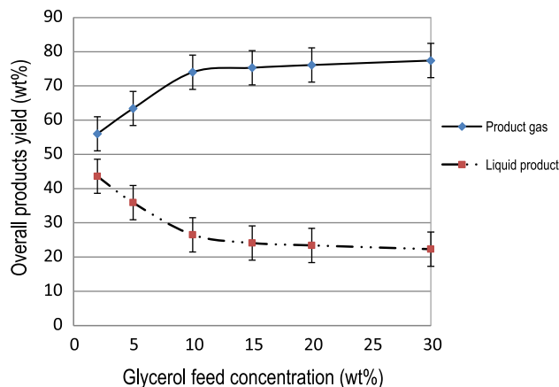
Fig. 11. Effect of glycerol concentration on gas-liquid product yields. T = 500 °C, 235 barg and WHSV = 125 h -1 .
