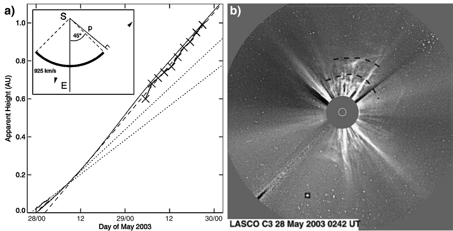
Fig. 8 (a) Distance-time plot of the May 2003 SMEI event from Tappin et al. (2004). Units of elongation have been converted to distance in AU using the Point P approximation ( r \sim \sin \varepsilon ), i.e., it is the perpendicular distance from the LOS intersecting the leading edge assuming the measured CME feature is a large spherical shell centered on the Sun (insert, upper left). The dashed line shows the extension back to the Sun and forward to beyond 1 AU. The solid curve is the extrapolation for a structure extending to 45^\circ from the Sun-Earth line and traveling at 925 km/s, shown schematically in the insert. (b) LASCO C3 coronagraph image of the associated CME, which is actually two CMEs launching in quick succession (black dashed arcs). Their distance-time plots are also shown by the dotted lines in panel (a)
