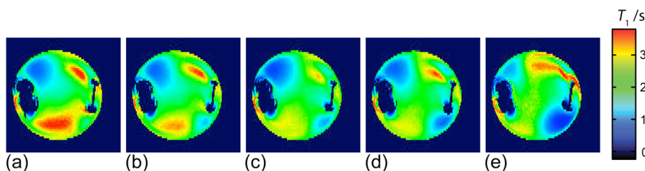
Figure 5. Horizontal 1 H MRI T_1 maps of the full Zn–air cell under constant load discharge at 12 k \Omega . Experiment conducted close to complete cell failure. Images were acquired upon connection (a), 11 h (b), 23 h (c), 30 h (d) and 47 h (e). The Zn strip is on the right. MRI parameters are the same as in Figure 3.
