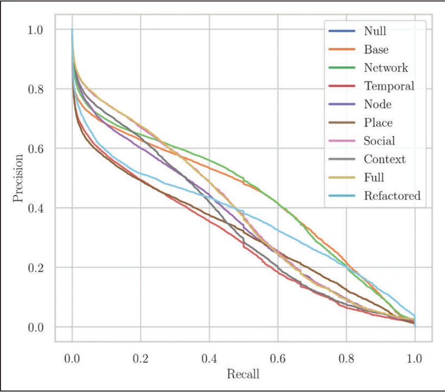
Figure 1. Precision recall curves. The figure depicts the precision-recall curves of the different models. As we fitted a separate tree R for each student, these curves were built by averaging the individual PR curves of each R . The network model performed best, while the base model was only slightly worse overall; in particular those two models managed to keep a relatively high precision score for higher recall values. The social and full model had relatively high precision scores as well.
