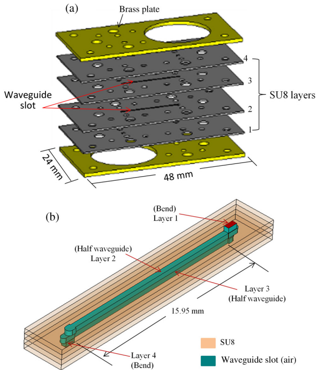
Fig. 1 Illustration of WR-3 waveguide structure with the right angle bends: (a) three-dimensional structure of the device and (b) the waveguide structure where the blue represents air in the reality.
