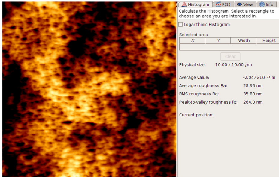
Fig. 9 Surface roughness of evaporated silver measured by atomic force microscopy.
