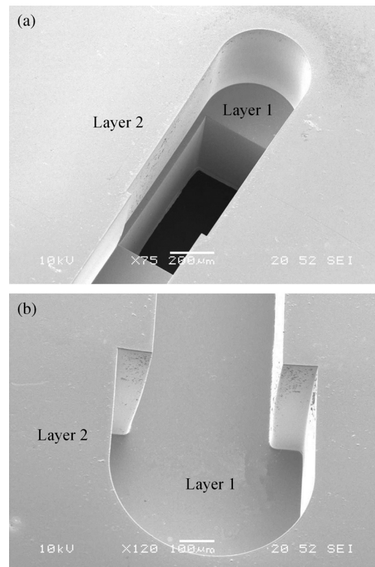
Fig. 5 Details of the waveguide bend formed by the two layers SU8 process. (a) Close view of the right-angle bend in layer 1 and excellent alignment between the two layers, (b) small angles along the sidewall in layer 2 due to the shadowing effect.
