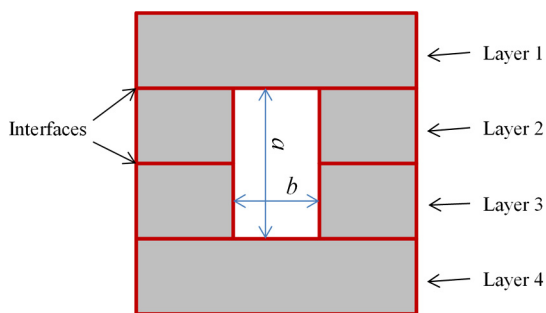
Fig. 2 Cross-sectional view of the WR-3 waveguide which consists of four layers. Each layer is designed as 432\text{-}\mu\text{m} thick. a = 864\text{ }\mu\text{m} and b = 432\text{ }\mu\text{m} . The red stands for the silver metallization.
