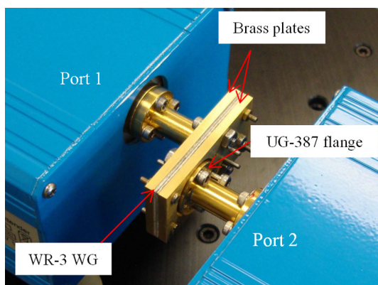
Fig. 7 Configuration of the measurement for the double-layered SU8 WR-3 waveguide.
