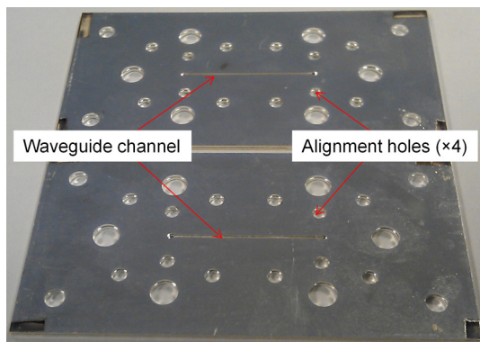
Fig. 4 Photo of silver-coated WR-3 waveguide halves. The size of both halves is 48 mm \times 24 mm \times 0.864 mm.
