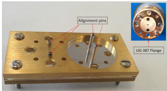
Fig. 6 Assembly of the WR-3 waveguide and the fitting of the measurement port.
