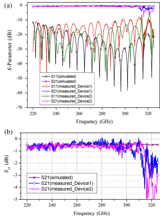
Fig. 8 (a) Measured S_{21} and S_{11} performance of the double-layered SU8 WR-3 waveguides comparing with the simulation results. (b) is a zoom-in view of S_{21} . The simulation employs an effective conductivity of 1.86 \times 10^7 S/m.
