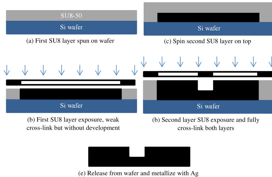
Fig. 3 Schematic diagram of the double-layer SU8 fabrication process.
