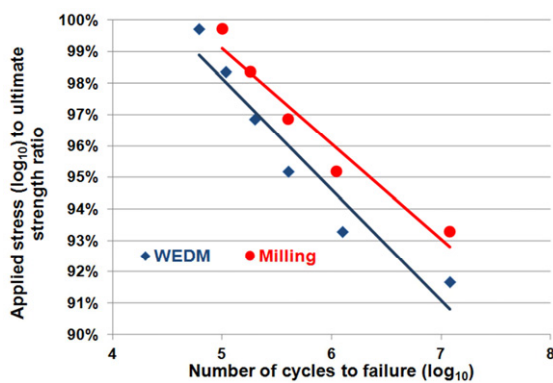
Fig. 5. \log_{10} - \log_{10} fatigue curve plots for Ti6246 specimens
