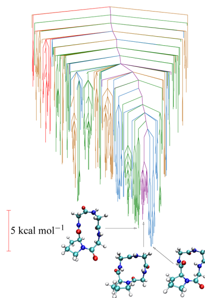
Figure 10. Disconnectivity graph showing the energy landscape of cyclo-[Gly 3 Pro] in water including the 358 minima and 2472 transition states accessible via transition states lower than 30 kcal mol -1 from the global minimum. Minima are colored by the number of trans-peptide groups from red (0) to purple (4).
