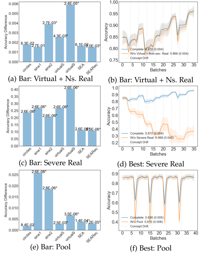
Fig. 9: Accuracy improvements obtained by each of OGMMF-VRD’s mechanisms. Each bar represents the subtraction of the average of the complete system from the average of the system without a given mechanism (e.g. w/o non-severe drift adaptation). The number above each bar represents the p-value obtained by Wilcoxon test over the comparison pair to pair. P-values representing statistically significant difference at the level of \alpha = 0.05 are marked by *. The AOT plots represent the dataset with the best improvement in each bar plot. The blue line represents the complete OGMMF-VRD system and the orange line represents the system without the respective mechanism.
