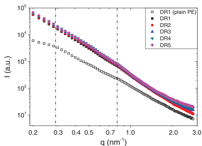
FIGURE 3 SAXS profile of gold/UHMWPE nanocomposite films normalized by the thickness for all samples under study including the DR 1 in the absence of Au nanoparticles [Color figure can be viewed at wileyonlinelibrary.com ]
