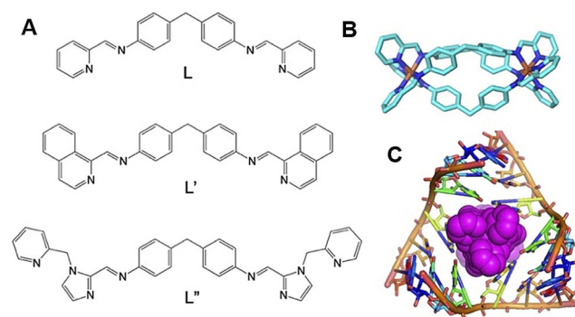
Figure 1. A) Structure of the ligands used in this study. B) Structure of the [\text{Ni}_2\text{L}_3]^{4+} cylinder of ligand L, [35] L', [36] and L'' [37] form analogous cylinders that bear further aryl rings on their external surfaces. C) View of the crystal structure of a cylinder bound in an RNA 3-way junction cavity from PDB 4J1Y [32] showing its unique binding.
