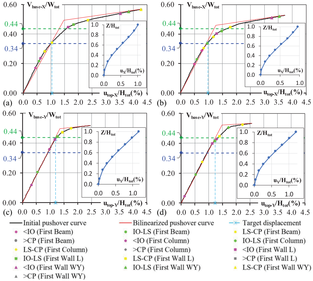
Figure 5. Critical normalized pushover curves of the Building along with notation for events for the load combinations (a) E_x + 0.3E_y , (b) -E_x - 0.3E_y , (c) -E_x + 0.3E_y , and (d) -E_y - 0.3E_x , where x and y are the directions of the Building.
