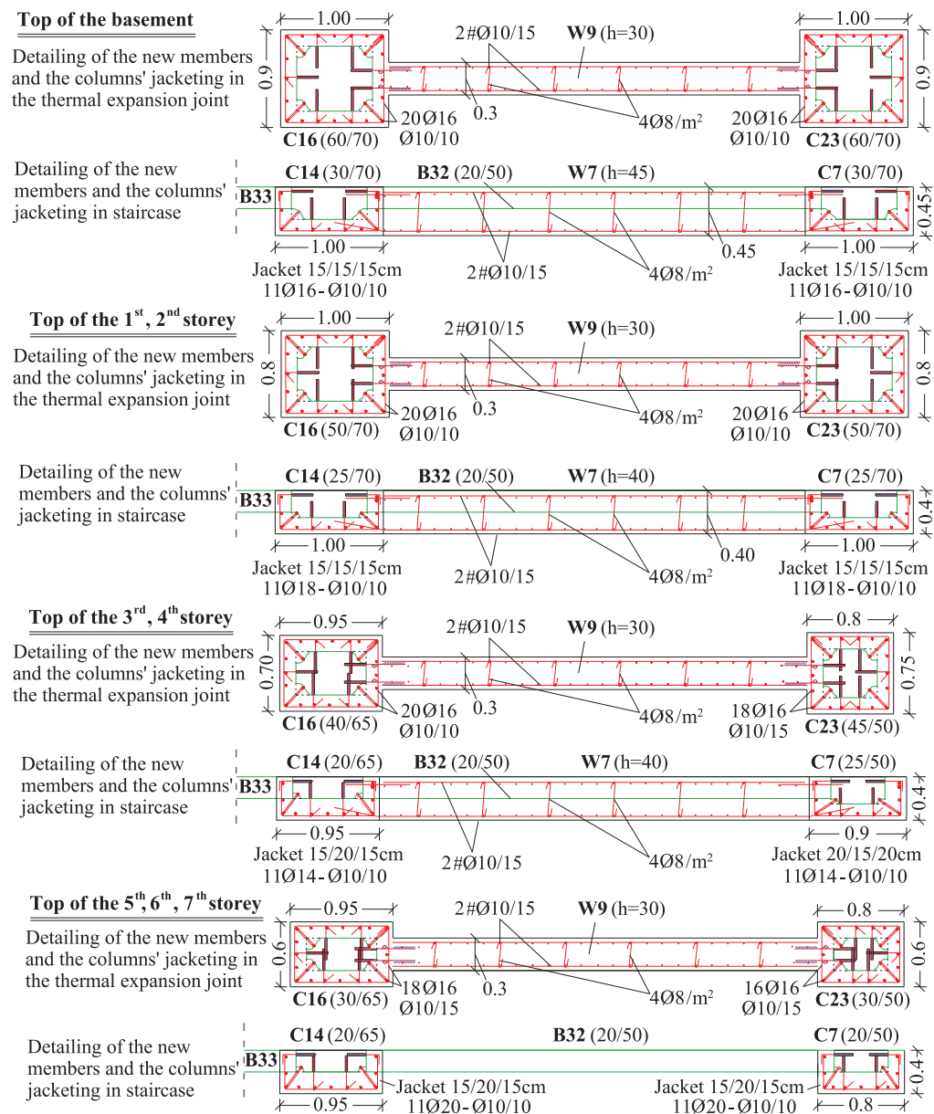
Figure 15. Detailing of the new r/c shear wall, members columns jacking of the solution RS3 for all floor levels.
