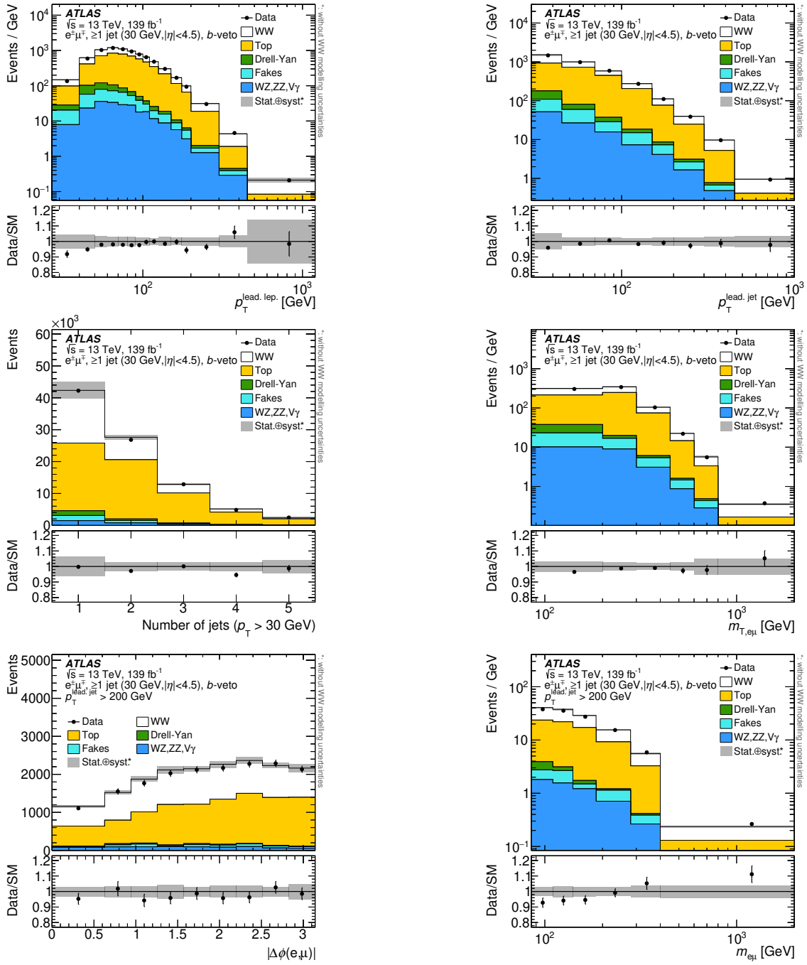
Figure 3. Signal region detector-level distributions of the p_T^{\text{lead. lep.}} (top left), the p_T^{\text{lead. jet}} (top right), the jet multiplicity (middle left), the m_{T,e\mu} (middle right), and, for events with p_T^{\text{lead. jet}} > 200 GeV, the \Delta\phi(e,\mu) (bottom left) and m_{e\mu} (bottom right). Data are shown as black markers together with the predictions for the signal and background production processes. The last bin contains overflow events. The lower panels show the ratio of the data to the total prediction. The uncertainty bands shown include statistical and systematic uncertainties, excluding theory uncertainties on the signal.
