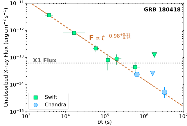
Figure 3. The Swift /XRT (green squares) and Chandra /ACIS-S (blue circles) unabsorbed X-ray flux light curve (0.3 – 10 keV) for GRB 180418A. Each observation is log-centered with the time errors denoting the duration of each observation. The flux errors are 1\sigma . In some cases, the symbols are bigger than the errors. The Swift and Chandra 3\sigma upper limits are indicated with green and blue arrows, respectively. The dashed light brown line represents the best-fit single power-law model with \alpha_X = -0.98^{+0.12}_{-0.16} . The dotted horizontal grey line shows the unabsorbed X-ray flux level of X1, \sim 6.24 \times 10^{-14} \text{ erg cm}^{-2} \text{ s}^{-1} (see Table 1).
