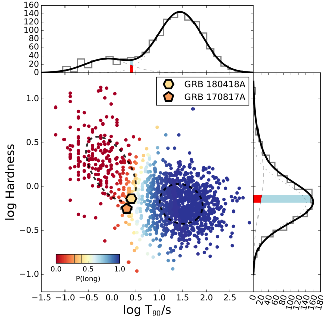
Figure 1. The Hardness- T_{90} (observer frame) plane of 1405 bursts detected by Fermi /GBM (Bhat et al. 2016). The color scale from red to blue indicates the probability that a given event is a long GRB ( P_{\text{long}} ), where a value of P_{\text{long}} = 0 indicates a short GRB. In the projected histograms for each parameter (top and right), the contributions from the short (red) and long (light blue) GRB populations at the position of GRB 180418A are shown, containing the classification based only on either duration or hardness alone. We use two 2-dimensional Gaussians to fit the distributions, where dashed-line ellipses correspond to 1\sigma confidence. The hexagon and pentagon indicate the locations of GRB 180418A and GRB 170817A, respectively. The position of each source has also been indicated with black lines in the probability color bar.
