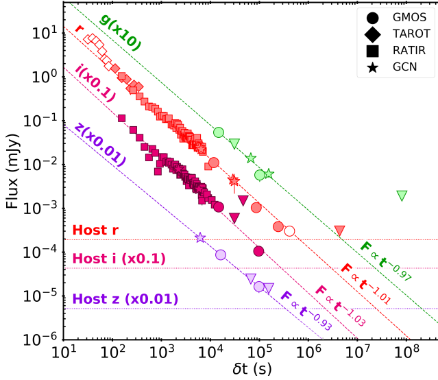
Figure 5. Optical afterglow light curves of GRB 180418A in the griz filters. Circles represent our new Gemini afterglow data (Table 2). Literature data from TAROT (diamonds), RATIR (squares) and other sources (stars) are also shown (Becerra et al. 2019; Choi et al. 2018; Guidorzi et al. 2018; Horiuchi et al. 2018; Malesani et al. 2018; Misra et al. 2018; Schady 2018; Schady & Chen 2018; Sota et al. 2018; Xin et al. 2018). Triangles indicate 3\sigma upper limits. Only those observations in the riz filters for which the host galaxy contribution is less than 5% of the total optical flux are plotted. Observations in the r -band which are ignored in the power-law fit are shown as open symbols. Horizontal lines denote the flux of the host galaxy, while dashed lines indicate the best-fit power-law decay models for the different bands.
