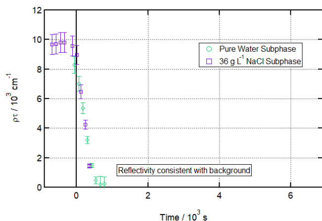
Figure 1. Ozonolysis of an oleic acid monolayer floating on pure vs. salt water. Time evolution plot for ozonolysis of 29 \mu\text{L } 1.0 \text{ g L}^{-1} d_{34}\text{-OA} ( \text{CHCl}_3 spreading solution) on pure water (green circles) and 25 \mu\text{L } 1.0 \text{ g L}^{-1} d_{34}\text{-OA } 36 \text{ g L}^{-1} \text{ NaCl(aq)} (purple squares) subphases by 323 \pm 29 \text{ ppb O}_3 introduced at t = 0 \text{ s} at 21 \pm 1 \text{ }^\circ\text{C} .
