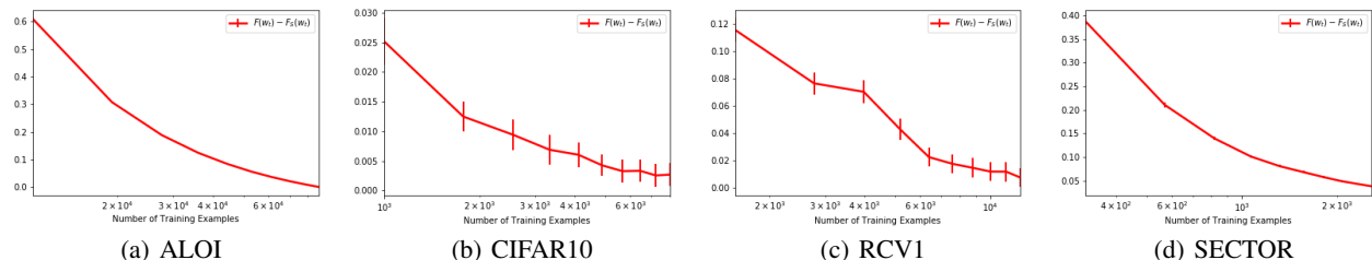
Figure 3: F(w_T) - F_S(w_T) versus the training data size.
