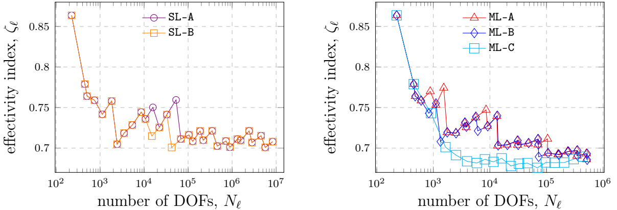
FIGURE 1. Experiments in section 7.1.1: Effectivity indices \zeta_\ell for the error estimates \tau_\ell in the SGFEM approximations generated by single-level (left) and multilevel (right) adaptive algorithms.
