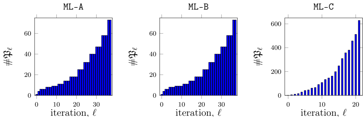
FIGURE 7. Experiments in section 7.2: Evolution of the cardinality of the index set \mathfrak{P}_\ell .
