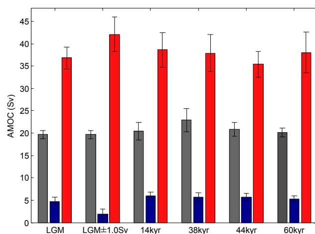
Fig. 1. 30 yr mean \pm 1 standard deviation Atlantic meridional overturning circulation (AMOC) values for the three phases of each climate simulation: grey for EQ (equilibrium), blue for HS (Heinrich stadial-like) and red for GI (Greenland interstadial-like).
