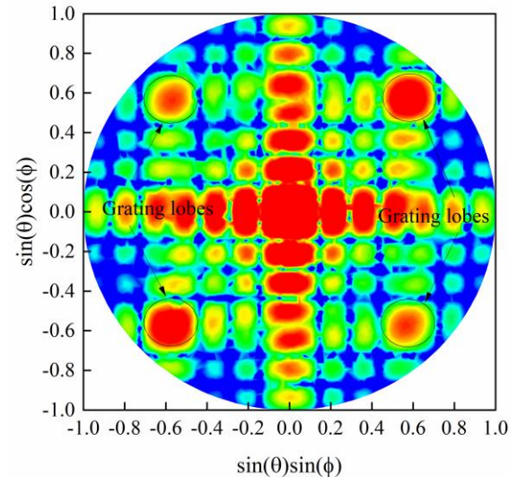
Fig. 4. Simulated 3-D radiation pattern of 4x4 sub-arrays based on Type I at the center frequency.
