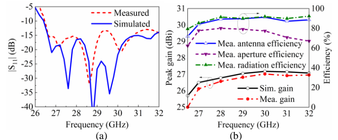
Fig. 13. (a) Simulated and measured reflection coefficient; (b) Simulated and measured peak gain and antenna efficiency.
