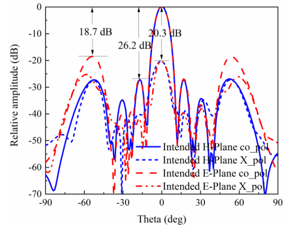
Fig. 5. Simulated 2-D radiation patterns of 4x4 sub-arrays based on Type I at the center frequency.
