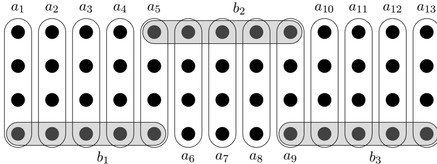
FIGURE 1. An example of an AB -set with k_A = 4 and k_B = 5 . The B -edge is shaded in grey.
