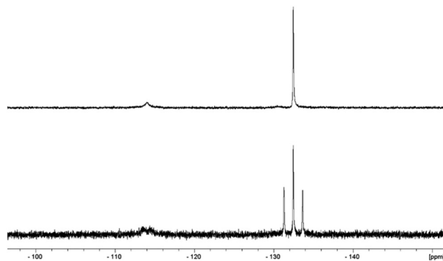
Fig. 4 ^{31}\text{P}\{^1\text{H}\} (top) and ^{31}\text{P} (bottom) NMR spectra (in d_8 -THF) of the reaction between 1 and BnK in the presence of 18-crown-6.
