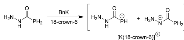
Scheme 4 Reaction of 1 , one equivalent of BnK and 18-crown-6 to yield [\text{K}(\text{18-crown-6})][\text{3}] .
