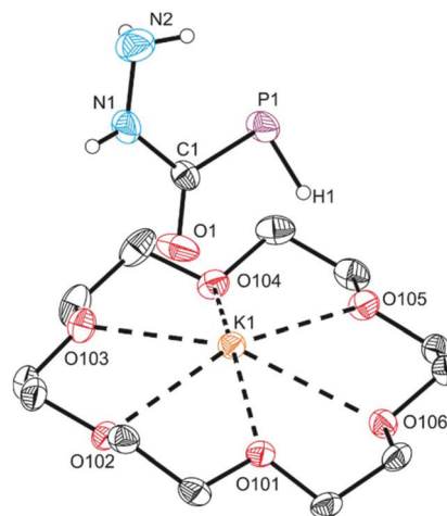
Fig. 6 Molecular structure of [\text{K}(\text{18-crown-6})][\textit{cis-cis-3a}] . Thermal ellipsoids pictured at the 50% probability level. Selected bond distances (Å) and angles (deg): P1–C1: 1.792(2) ; C1–O1: 1.248(3) ; C1–N1: 1.383(3) ; N1–N2: 1.393(3) ; O1–K1: 2.679(2) ; O1–C1–P1: 128.0(2) ; N1–C1–P1: 115.26(18) ; O1–C1–N1: 116.7(2) ; C1–N1–N2: 122.8(2) .
