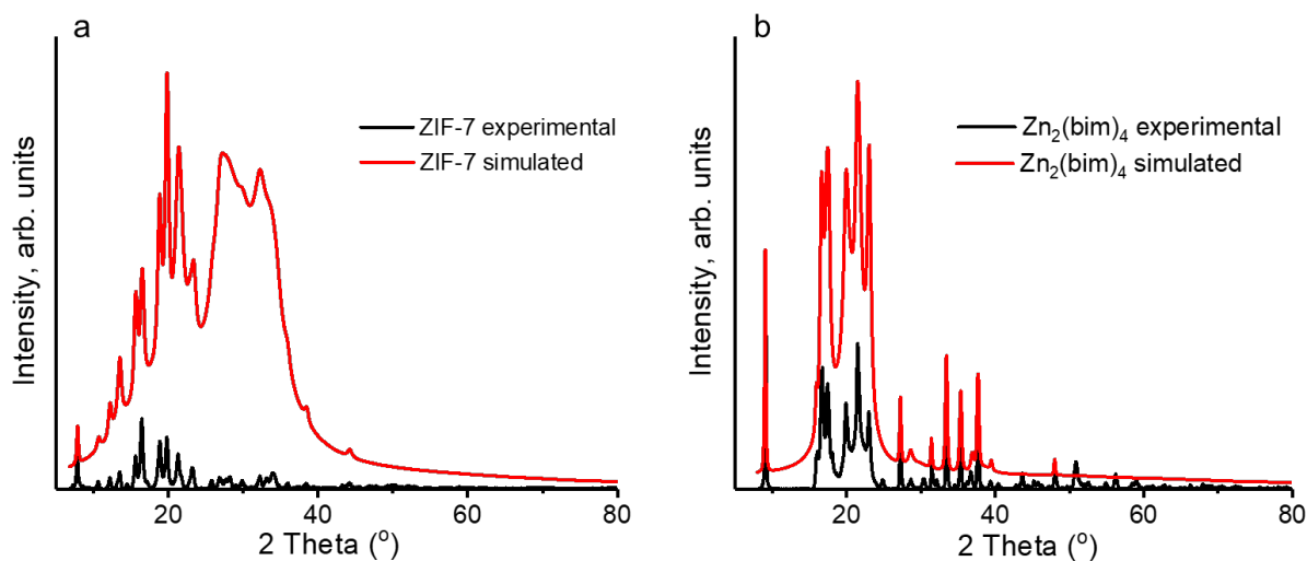
Figure 2. XRD pattern of the synthesized (a) ZIF-7 and (b) \text{Zn}_2(\text{bim})_4 particles. Red curves show the PXRD simulated patterns.
