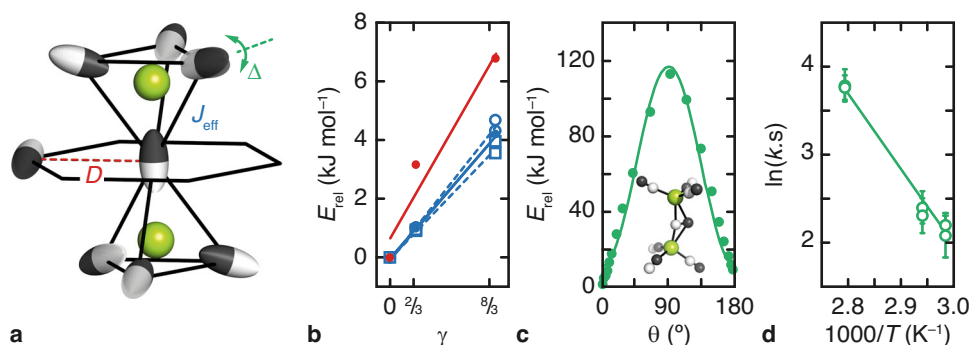
Fig. 3 Microscopic single-ion and pairwise interaction parameters in \text{Cd}(\text{CN})_2 . a The effective exchange interaction (strength J_{\text{eff}} ) operates between nearest neighbours within the same pyrochlore sublattice. Dipolar interactions (strength D ) give rise to an effective exchange interaction between nearest neighbours on alternate sublattices. The single-ion anisotropy term \Delta reflects the enthalpy barrier to \text{CN}^- reorientations. b Relative DFT energies E_{\text{rel}} for a series of single network (filled blue symbols) and interpenetrated (filled red symbols) \text{Cd}(\text{CN})_2 configurations with different \text{CdC}_n\text{N}_{4-n} coordination environments: \text{CdC}_2\text{N}_2 (geometric parameter \gamma = \frac{2}{3}(n-2)^2 = 0 ), \text{CdC}_3\text{N}/\text{CdCN}_3 ( \gamma = \frac{2}{3} ) and \text{CdC}_4/\text{CdN}_4 ( \gamma = \frac{8}{3} ). Simple geometric arguments give E_{\text{rel}} = \gamma J_{\text{eff}} and \gamma(J_{\text{eff}} + D) for single-network and interpenetrated \text{Cd}(\text{CN})_2 , respectively. The corresponding NMR-derived values are shown with open blue symbols (squares = ref. 34 circles = this study). c Nudged elastic band calculation energies for a 180^\circ \text{CN}^- orientation flip (filled green symbols) and corresponding fit E_{\text{rel}}(\theta) = \Delta \cos^2\theta = \Delta S_{\parallel}^2 (solid green line), from which the value of \Delta was obtained. The \Delta \simeq 90^\circ transition state involves a C-bridged Cd-(CN)-Cd linkage (inset) and a reduced Cd...Cd separation. d Arrhenius plot reflecting the temperature dependence of \text{CN}^- flipping rates as determined using ^{113}\text{Cd} EXSY spectroscopy. Error bars denote the standard error in rate constants determined extracted during fitting (see Supplementary Figure 6 and Supplementary Table 7). The experimental value of \Delta is given by the gradient of the linear fit (solid line).
