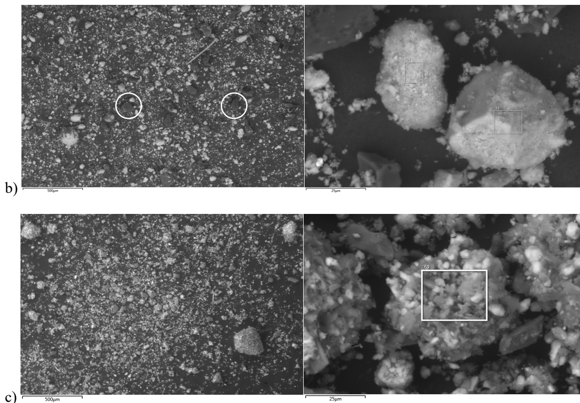
Figure 4 ESEM images of a) POW + Chem-NaHCO 3 , b) POW + Chem-CaO, and c) POW + Chem-Na 2 CO 3 -ZnO mixtures after pyrolysis in batch reactor at 480 °C for 3 h. High magnification ESEM images show examples of rectangular areas used in the chlorine determination by EDS.
