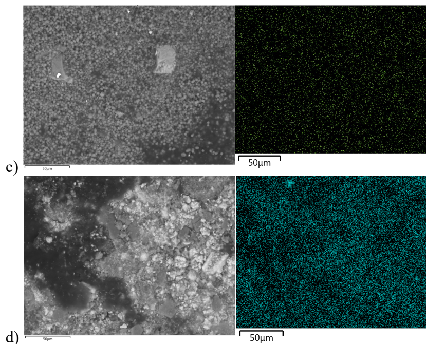
Figure 7 Chlorine mapping by ESEM-EDS (right-hand images) of a) Ads- \text{Al}_2\text{O}_3 -1; b) Ads- \text{Al}_2\text{O}_3 -2; c) Ads-NaX; and d) Chem- \text{Na}_2\text{CO}_3 -ZnO, after their use as a hot filter.
