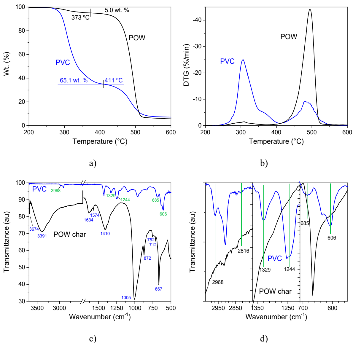
Figure 2 a) TGA and b) DTG profiles of POW and pure PVC in N 2 atmosphere at a heating rate of 10 °C/min. c) FTIR spectra of POW pyrolyzed to 480 °C and pure PVC. d) Zones of bands associated with C–H and C–Cl stretching in the –CHCl– groups for POW char and pure PVC.
