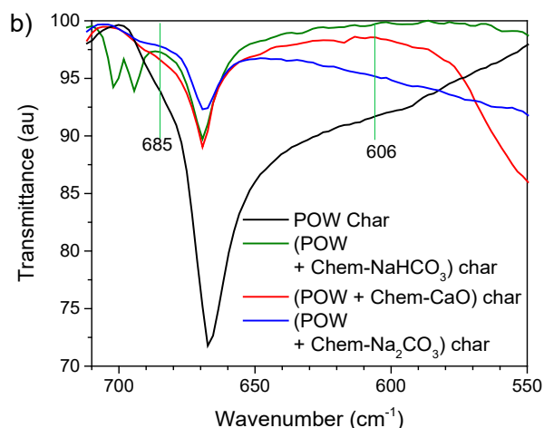
Figure 5 a) FTIR spectra for fresh chemical removers (without POW) and chars of mixtures after pyrolysis at 480 °C in the batch reactor; b) Zoom of the FTIR 710-550 \text{cm}^{-1} region of pyrolyzed mixtures. Lines in b) at 606 and 685 \text{cm}^{-1} represent the theoretical position of the C–Cl stretching in the –CHCl– groups.
