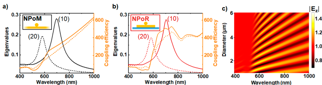
Figure 2. Enhanced light localization in nanocavities driven by an external resonator. (a, b) Eigen-analysis of (a) NPoM and (b) NPoR plasmonic constructs. Eigenmodes of NPoM (black) and NPoR (red) and coupling efficiency (orange) for (20) (dashed) and (10) (solid) resonances. Insets show each plasmonic system. (c) Total electric field E_z from outward and reflected plasmons at the center of the disk for increasing disk diameters, D = 1\text{--}6 \mu\text{m} .
