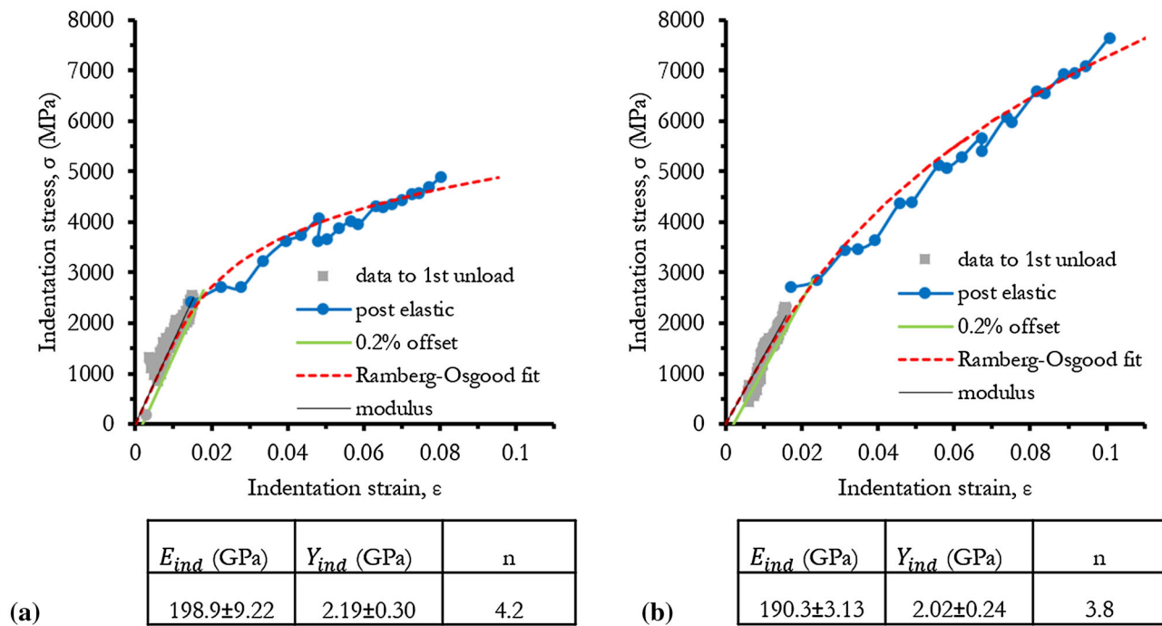
Fig. 13 Spherical nanoindentation stress–strain curves for (a) tube and (b) stent, showing indentation modulus, E_{ind} , yield stress defined by 0.2% indentation strain offset and Ramberg–Osgood fit
