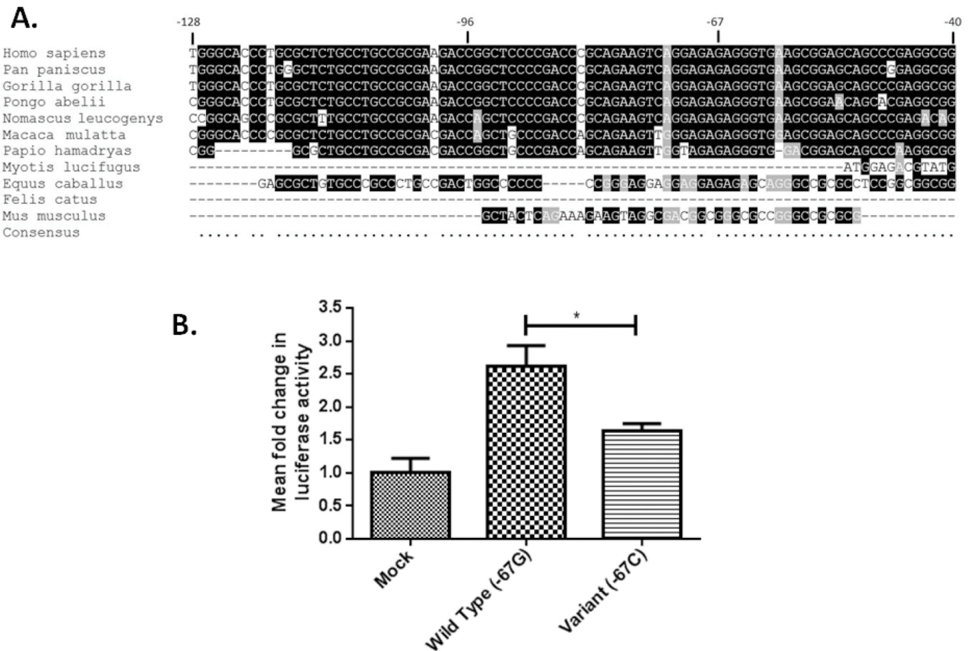
Fig 1. c.-67G>C in the 5'UTR of F2R alters transcriptional activity. (A) Alignment of F2R 5'UTR nucleotide sequences across multiple species, highly conserved nucleotides are highlighted in black. (B) HEK293T cells were transfected with 200 ng of either -67G or -67C F2R luciferase reporter construct, or an empty vector control. Forty-eight hours post-transfection, cells were lysed and luciferase activity assessed. Luciferase levels were normalised for transfection efficiency using Renilla activity. Data shown represents three independent experiments with a minimum of 3 technical replicates to calculate mean fold change \pm SE. (* p < 0.05 ).
