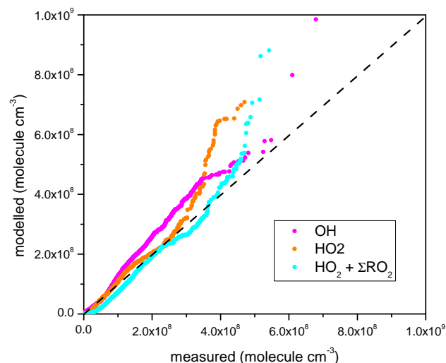
Fig. 9. QQ plot showing simultaneous modelled and measured OH (magenta), HO 2 (orange) and (HO 2 + ΣRO 2 ) (cyan) concentrations. OH data are multiplied by 100, HO 2 by two and (HO 2 + ΣRO 2 ) is divided by 3. A 1-1 line is shown for comparison.
