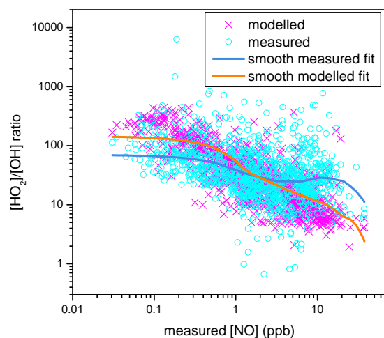
Fig. 5. Modelled (magenta) and measured (cyan) \text{HO}_2 :OH ratios plotted against measured NO concentrations. Data are shown as 15-min averages for direct comparison. Also shown are smoothed fits through each data-set (see text).
