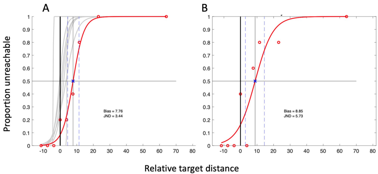
Fig. 7 The individual reach-estimate psychometric fits of the older control group (grey curves) and IW (red curve and data points) for the dominant arm a and, for IW only, the non-dominant arm b . The horizontal axis is target distance relative to actual reach distance (thick black vertical line), presented as percentage of arm length. The
