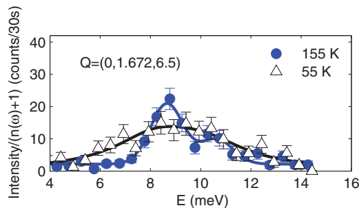
FIG. 6. (Color online) IXS E scan of the low-energy phonons at Q = (0,1.672,6.5) for T = 55 and 155 K. Phonons are fitted to a damped harmonic oscillator (DHO) response function (solid lines). Fits are convolved with the instrumental resolution.
