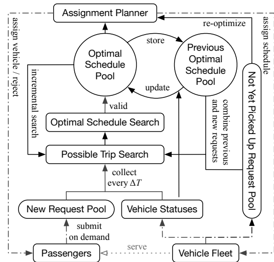
Fig. 2: Framework of the dispatch logic.
