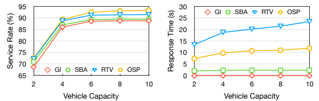
Fig. 3: Performance comparison during the whole day for varying capacity \kappa .
