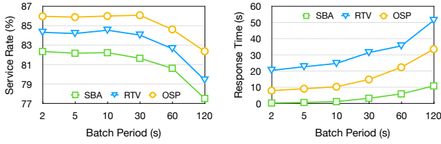
Fig. 5: Performance comparison during the peak hour for varying batch period \Delta T .
