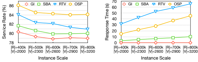
Fig. 6: Performance comparison during the peak hour for varying instance scale.
