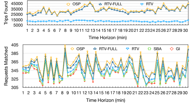
Fig. 7: Number of feasible trips found for all vehicles (upper plot) and number of matched new submitted requests (lower plot) at different dispatch epochs ( |R| = 800k , |V| = 3200 , \kappa = 8 , \Omega = 300 s, \Delta T = 30 s).
