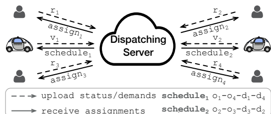
Fig. 1: Architecture of an SAMoD system with two vehicles and four requests, where vehicle 1 is assigned to serve requests 1&4 following schedule 1 ( o_i : pick up request r_i , d_i : drop off r_i ) and vehicle 2 is assigned to serve requests 2&3 following schedule 2.
