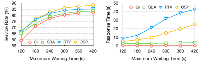
Fig. 4: Performance comparison during the peak hour for varying maximum waiting time \Omega .
