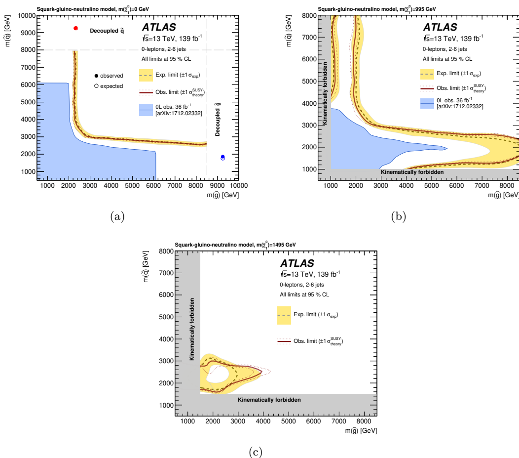
Figure 17. Exclusion limits for the model with combined production of squark pairs, gluino pairs, and squark-gluino pairs, for different \tilde{\chi}_1^0 assumptions about the neutralino mass: (a) m(\tilde{\chi}_1^0) = 0 GeV, (b) m(\tilde{\chi}_1^0) = 995 GeV and (c) m(\tilde{\chi}_1^0) = 1495 GeV, varying values of m(\tilde{g}) and m(\tilde{q}) and assuming a purely bino \tilde{\chi}_1^0 . Exclusion limits are obtained by using the signal region with the best expected sensitivity at each point. Observed limits are indicated by the medium dark (maroon) curves where the solid contour represents the nominal limit, and the dotted lines are obtained by varying the signal cross-section by the renormalisation and factorisation scale and PDF uncertainties. The expected limits are indicated with dark dashed curves, with the light (yellow) bands indicating the 1\sigma excursions due to experimental and background-only theoretical uncertainties. In figure (a) observed and expected limits on squark (gluino) masses are also shown, assuming gluino (squark) masses are decoupled as in simplified models presented in figure 13 (14). Results (a) and (b) are compared with the observed limits obtained by the previous ATLAS searches with no leptons, jets and missing transverse momentum [13].
