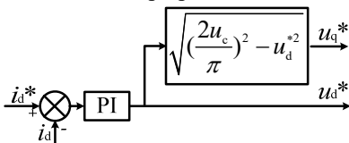
Fig. 3. Single current regulator control in six-step operation
