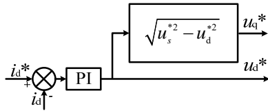
Fig. 2. Modified CCR-VQV flux-weakening control
