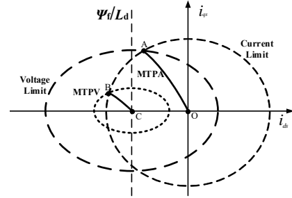
Fig. 4. Working areas of PMSM
