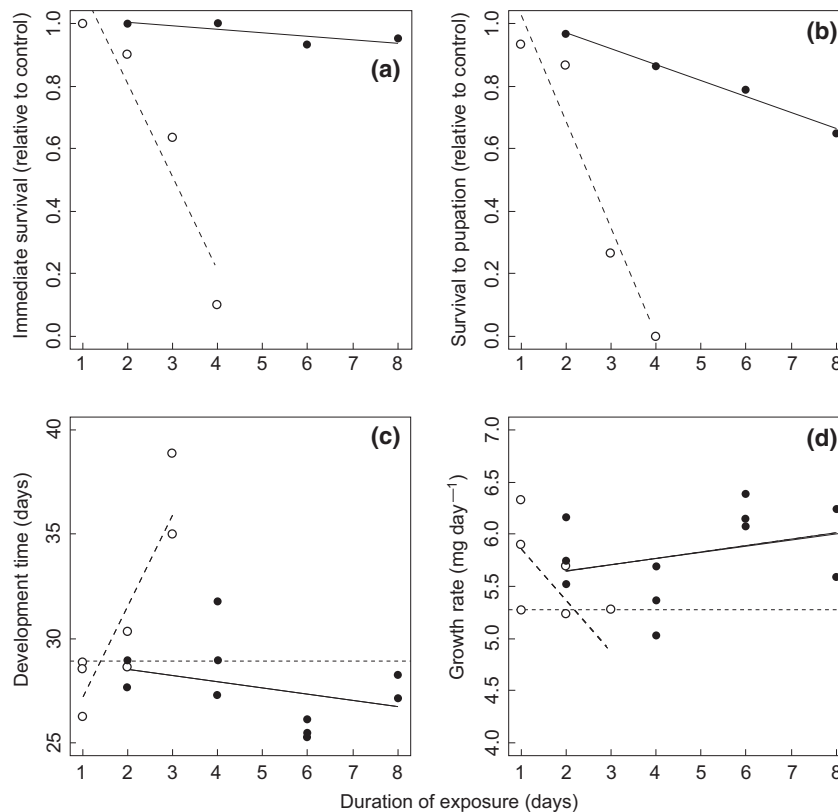
Fig. 3 Lethal and sublethal effects of cold exposure on Pararge aegeria larvae in laboratory experiment. Solid lines and closed symbols are larvae exposed to -5^{\circ}\text{C} , and long dashed lines and open symbols are larvae exposed to -10^{\circ}\text{C} . (a) Survival 2 days after stress treatment was terminated; (b) survival to pupation; (c) development time to pupation (days); and (d) growth rate (mg per day) following different cold exposure durations. For (a and b), survival rate is calculated as a proportion of survival rates of the control group. For (c and d) the horizontal short dashed lines show the average values for control groups.
