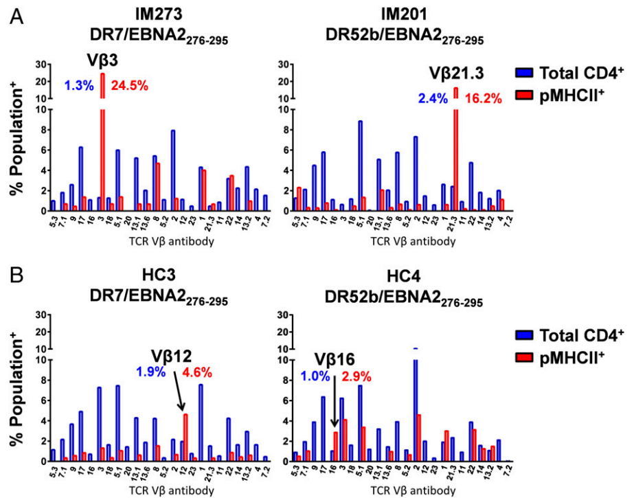
FIGURE 5. EBV-specific CD4 + T cells display biased TCR Vβ use in patients with IM. ( A and B ) CD4-enriched PBMCs from patients with IM ( A ) and healthy carriers (HC) ( B ) were stained with the indicated pMHCII tetramers and analyzed by flow cytometry for surface expression of defined TCR Vβ segments. Clonograms show the distribution of specific TCR Vβ segments among total CD4 + (blue) and EBV-specific pMHCII tetramer + CD4 + T cells (red). The dominant TCR Vβ segment is highlighted in each case.
