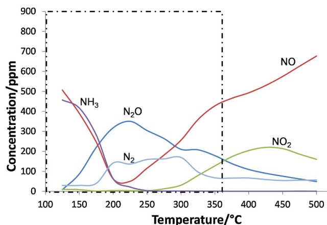
Fig. 6. NO x -reduction performance of V 2 O 5 -WO 3 /TiO 2 tested in a simulated exhaust gas containing NH 3 as reductant. Dotted line indicates typical 'temperature window' for diesel exhaust emitted by passenger cars.
