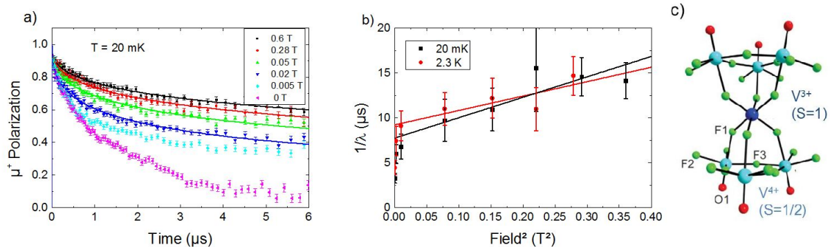
Figure 1. a) Time dependent muon spin polarization in DQVOF at 20 mK with different applied longitudinal fields. Solid lines are fits to the data (see text). b) Inverse of the relaxation rate versus field square. The solid lines are fits to the data. c) Local structure of the compound.
