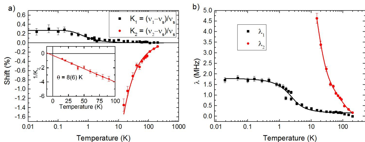
Figure 4. a) Shift versus temperature. K_1 relates to the narrow peak at high temperature and K_2 to the broad one. Inset : 1/K_2 versus temperature. The solid lines are fits to the data (see text). b) Depolarization rate versus temperature. \lambda_1 is relative to the narrow peak at high temperature and \lambda_2 to the broad one. Solid lines are guides to the eyes.
