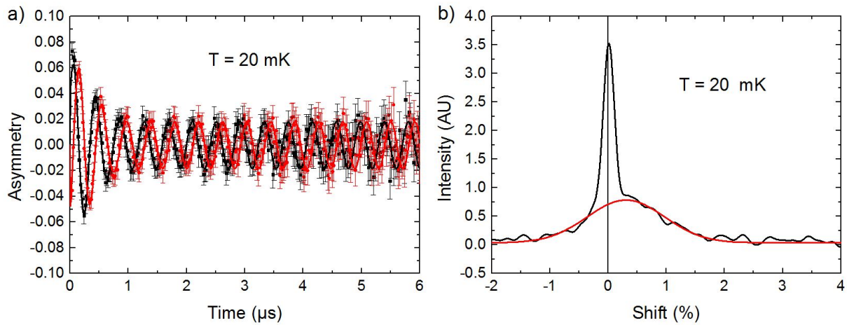
Figure 3. a) Time dependent signal at 20 mK with an applied transverse field of 0.5 T. The solid lines are fits to the data (see text). b) Fourier transform of the signal. The red line is a fit of the broad peak hidden under the silver narrow peak. The datas were taken on the LTF spectrometer
