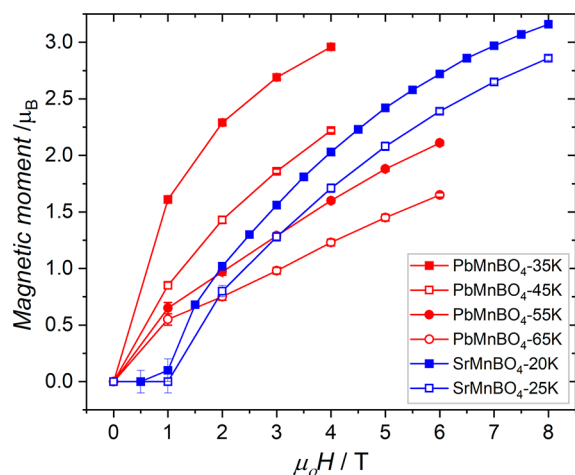
Figure 17. Variation of the FM magnetic moment induced by applied fields above the ordering temperatures of \text{PbMnBO}_4 and \text{SrMnBO}_4 .
