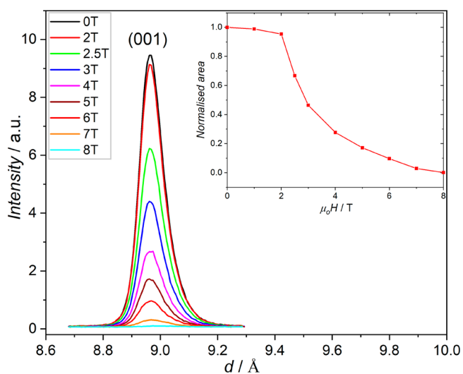
Figure 15. Change in intensity of the AFM (001) peak in \text{SrMnBO}_4 as a function of applied field at 1.5 K. The inset shows the change in integrated area with B .
