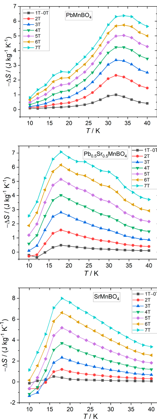
Figure 18. Magnetic entropy changes in \text{PbMnBO}_4 , \text{Pb}_{0.5}\text{Sr}_{0.5}\text{MnBO}_4 , and \text{SrMnBO}_4 when switching from zero to various applied fields.
