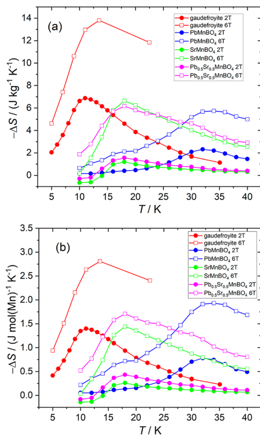
Figure 19. Comparison of magnetic entropy changes between 0–2 T and 0–6 T for gaufreyite, 17 \text{PbMnBO}_4 , \text{SrMnBO}_4 , and \text{Pb}_{0.5}\text{Sr}_{0.5}\text{MnBO}_4 (a) per kg sample and (b) per mol Mn.
