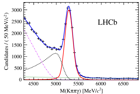
FIG. 1 (color online). Mass distribution of the selected B^+ \rightarrow K^+ \pi^- \pi^+ \gamma candidates. The blue solid curve shows the fit results as the sum of the following components: signal (red solid), combinatorial background (green dotted), missing pion background (black dashed), and other partially reconstructed backgrounds (purple dash-dotted).
