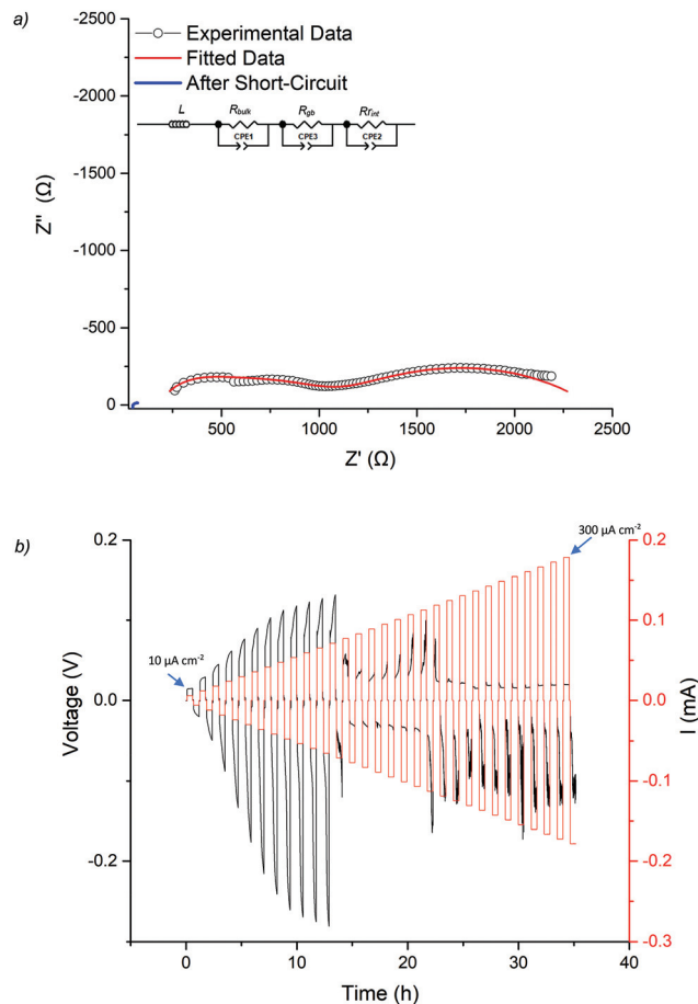
Fig. 6 (a) The impedance spectrum of the Li symmetry cell before and after CCD testing of Ga-LLHO at 21^\circ\text{C} , the fit at higher frequencies is representative of slightly overlapping bulk and grain components, hence was fit with two R/CPE components (b) CCD testing starting at 10 \mu\text{A cm}^{-2} and increasing in increments of 10 \mu\text{A cm}^{-2} until 300 \mu\text{A cm}^{-2} , with a large drop in voltage at 120 \mu\text{A cm}^{-2} indicating cell short circuit and lithium dendrite growth.
