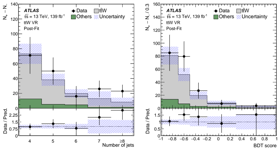
Figure 5: Post-fit comparison between data and prediction in the t\bar{t}W +jets validation region for the multiplicity of jets (left) and the BDT score (right). The y-axis label N_+ - N_- represents the difference between the number of events with a positive sum and the number of events with a negative sum of the charges of the selected leptons. The band includes the total uncertainty of the post-fit computation. The ratio of the data to the total post-fit computation is shown in the lower panel. The first and last bins contain underflow and overflow events, respectively.
