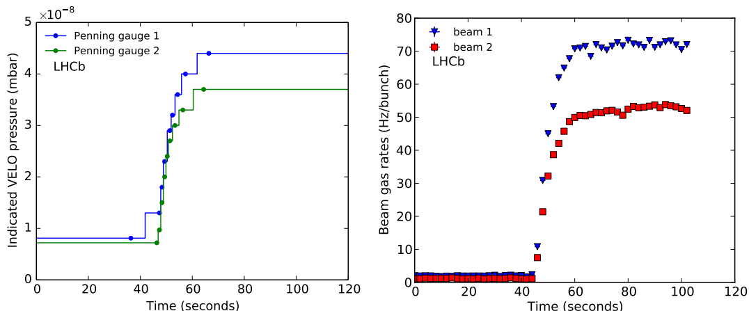
Figure 15. Effect of the gas injection (fill 2520), with (left) the pressure increase in the VELO and (right) the trigger rate increase. The VELO ion pumps are off. The pressure is measured with Penning gauges in the vacuum vessel within 50cm of the interaction point. The indicated value when neon is injected is to be multiplied by approximately a factor four to account for the lesser gauge sensitivity to neon gas. The absolute pressure increase cannot be accurately determined as the gas composition is unknown before the start of injection. The beam-gas rate for triggered events increases from about 2 to 72 Hz/bunch for beam 1 and 1.3 to 51 Hz/bunch for beam 2.
