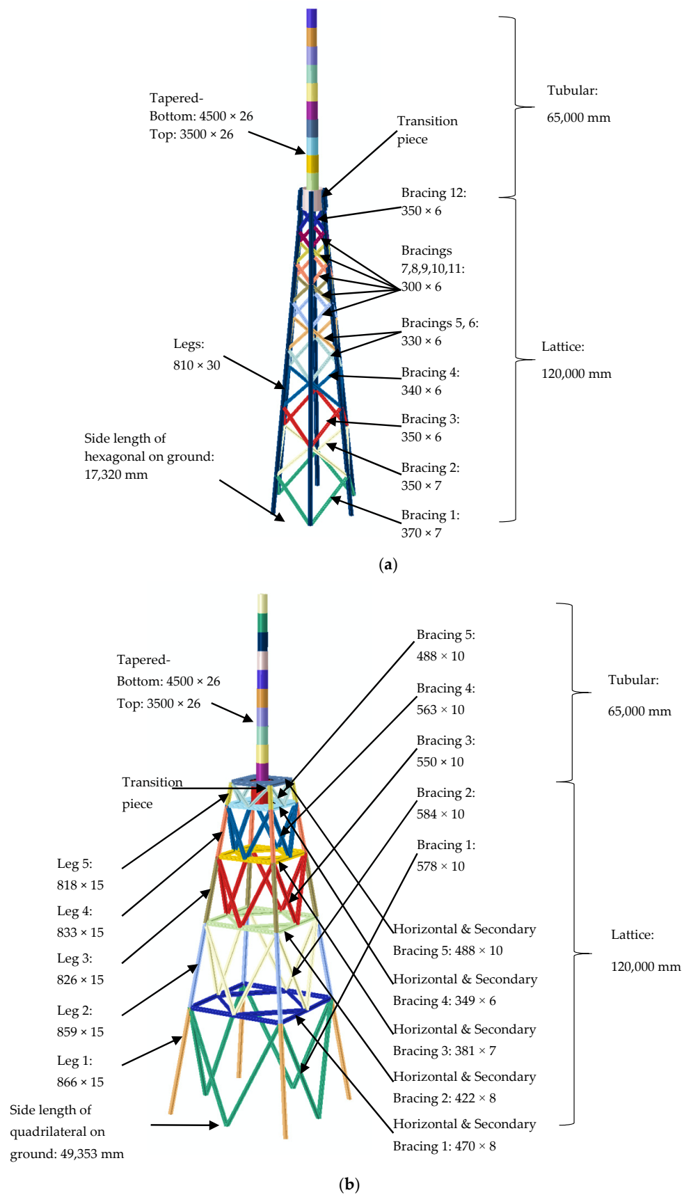
Figure 2. Case studies considered for LCA (dimensions in mm). (a) A 6-legged tower, (b) A 4-legged tower.
